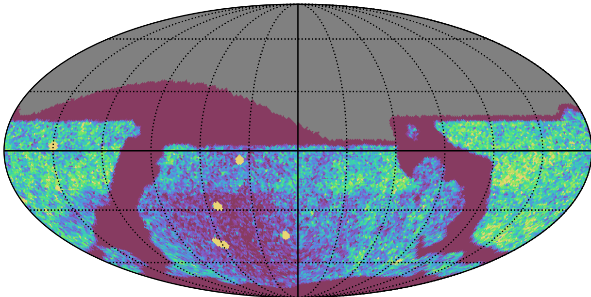
early_u_fpextra3.0_v3.4_10yrs Yr 1 all bands: NVisits
