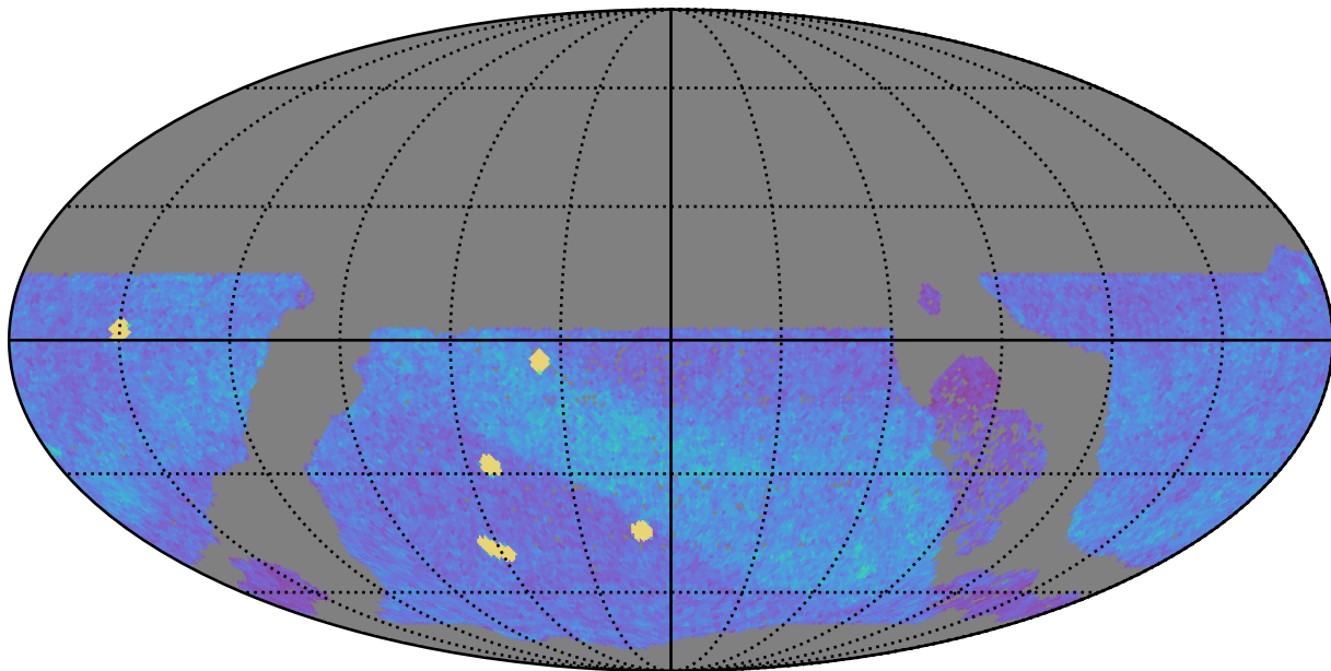
early_u_fpextra3.0_v3.4_10yrs WFD z band: NVisits
