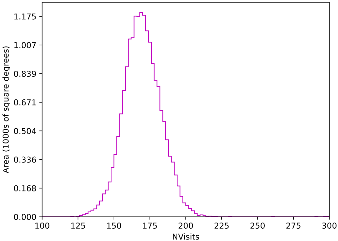
early_u_fpextra3.0_v3.4_10yrs WFD z band: NVisits
