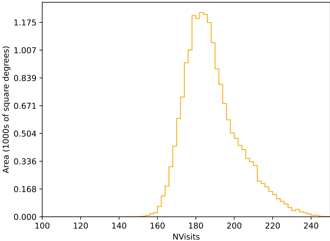
early_u_fpextra3.0_v3.4_10yrs WFD r band: NVisits
