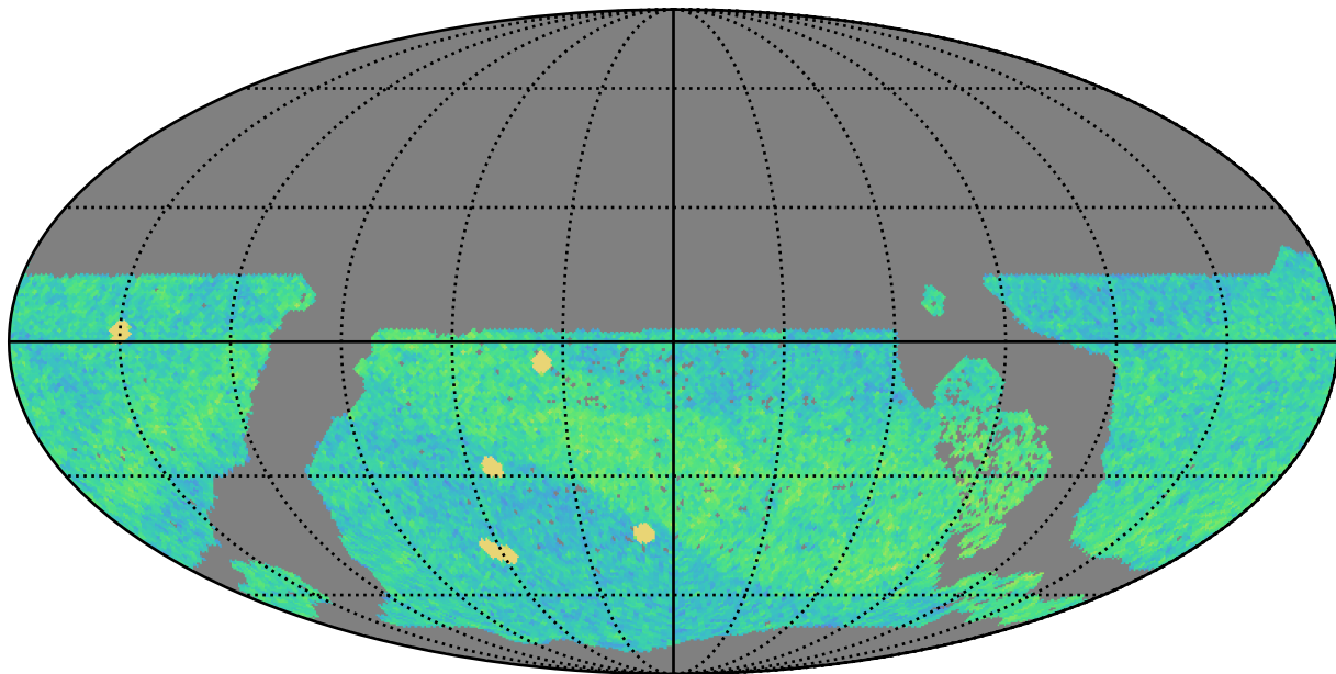
early_u_fpextra3.0_v3.4_10yrs WFD i band: NVisits
