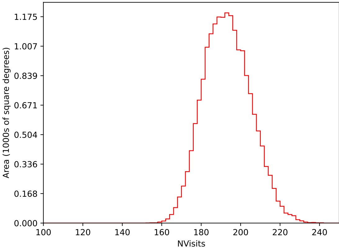
early_u_fpextra3.0_v3.4_10yrs WFD i band: NVisits
