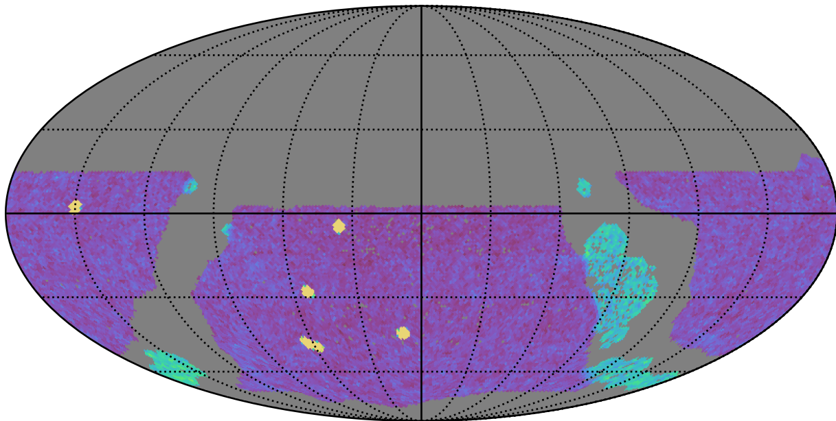
early_u_fpextra3.0_v3.4_10yrs WFD g band: NVisits
