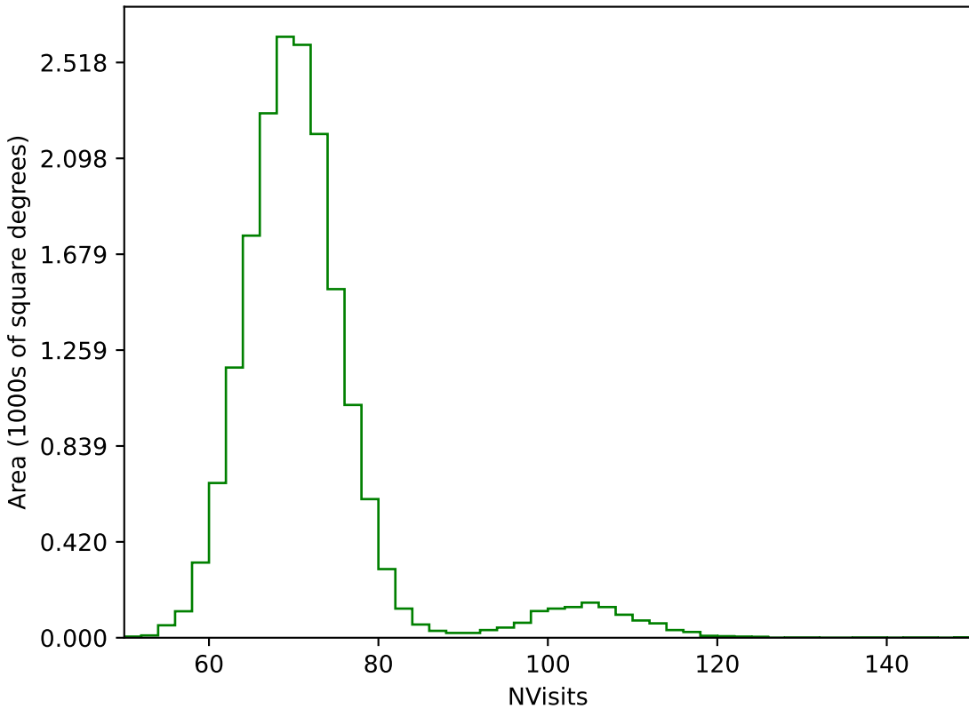
early_u_fpextra3.0_v3.4_10yrs WFD g band: NVisits
