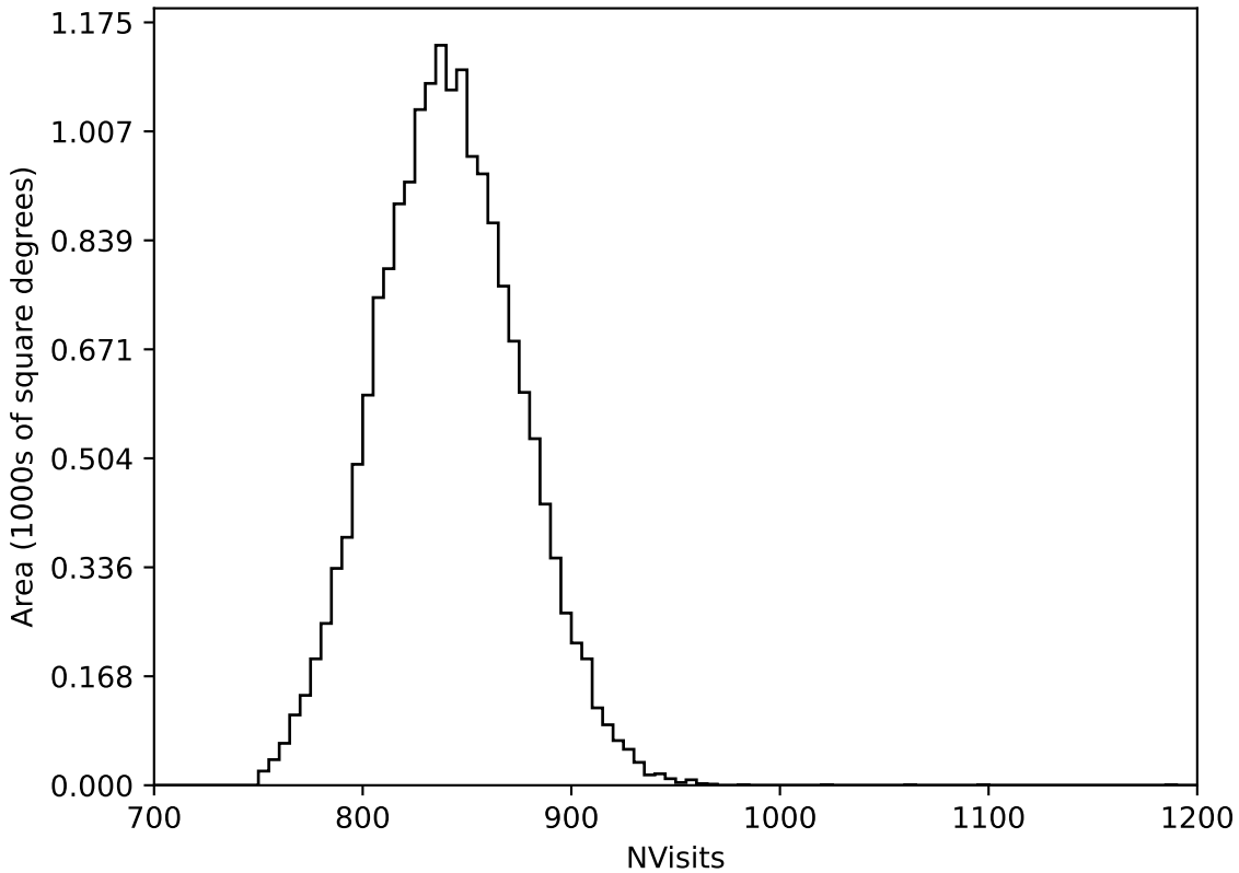
early_u_fpextra3.0_v3.4_10yrs WFD all bands: NVisits
