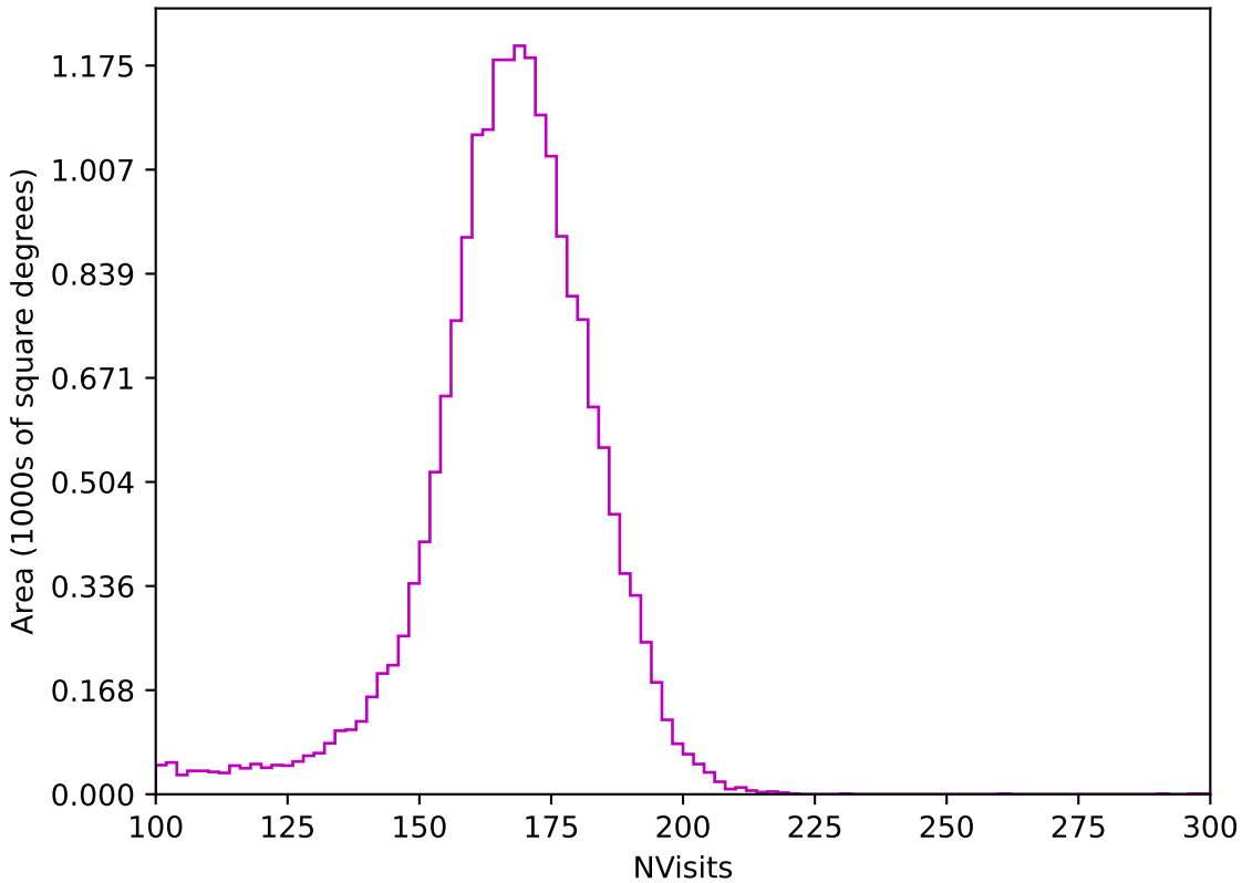
early_u_fpextra3.0_v3.4_10yrs All sky z band: NVisits
