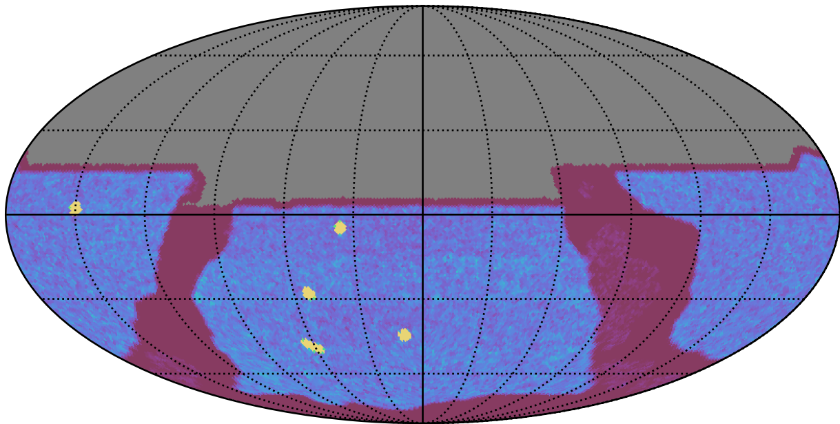
early_u_fpextra3.0_v3.4_10yrs All sky y band: NVisits
