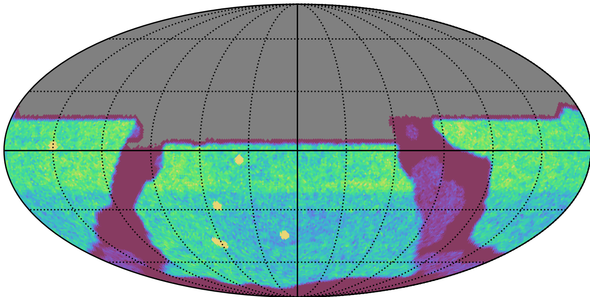
early_u_fpextra3.0_v3.4_10yrs All sky u band: NVisits
