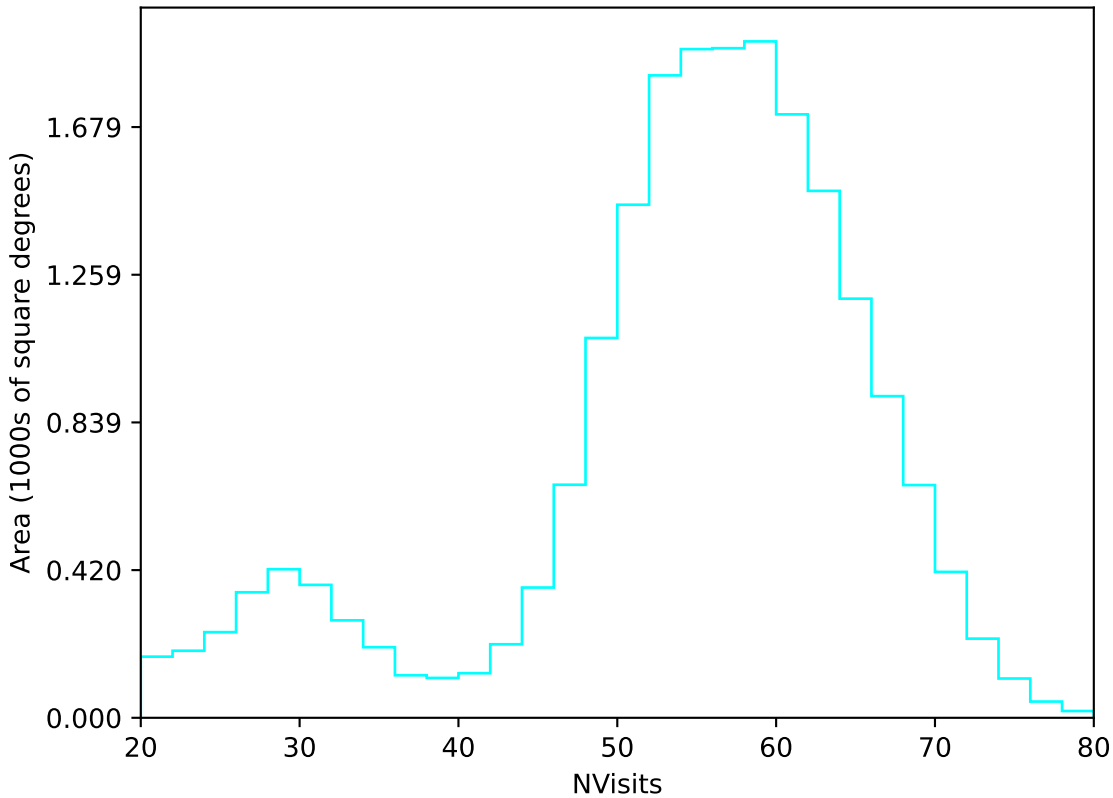
early_u_fpextra3.0_v3.4_10yrs All sky u band: NVisits
