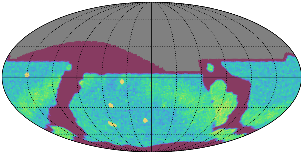
early_u_fpextra3.0_v3.4_10yrs All sky r band: NVisits
