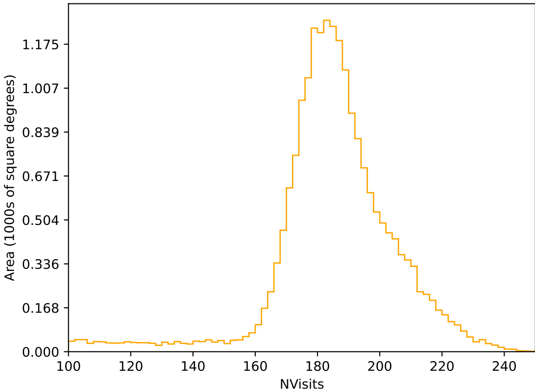
early_u_fpextra3.0_v3.4_10yrs All sky r band: NVisits
