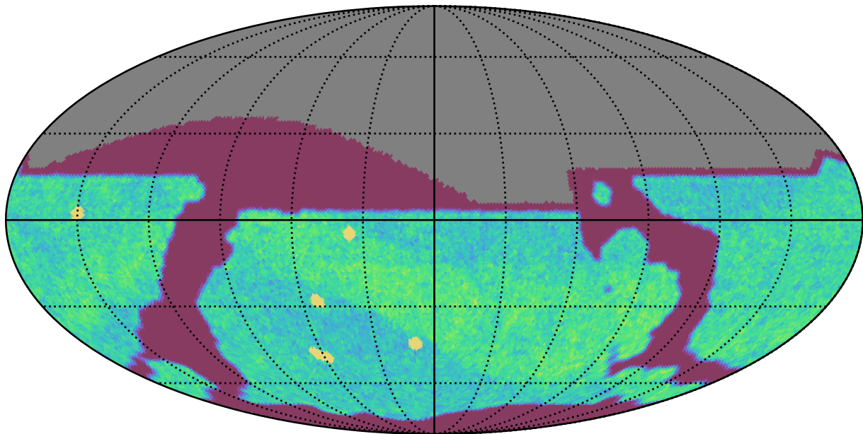
early_u_fpextra3.0_v3.4_10yrs All sky i band: NVisits
