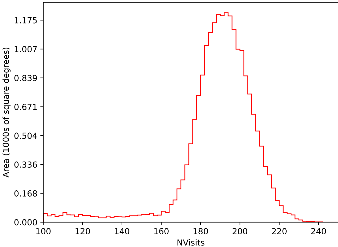
early_u_fpextra3.0_v3.4_10yrs All sky i band: NVisits
