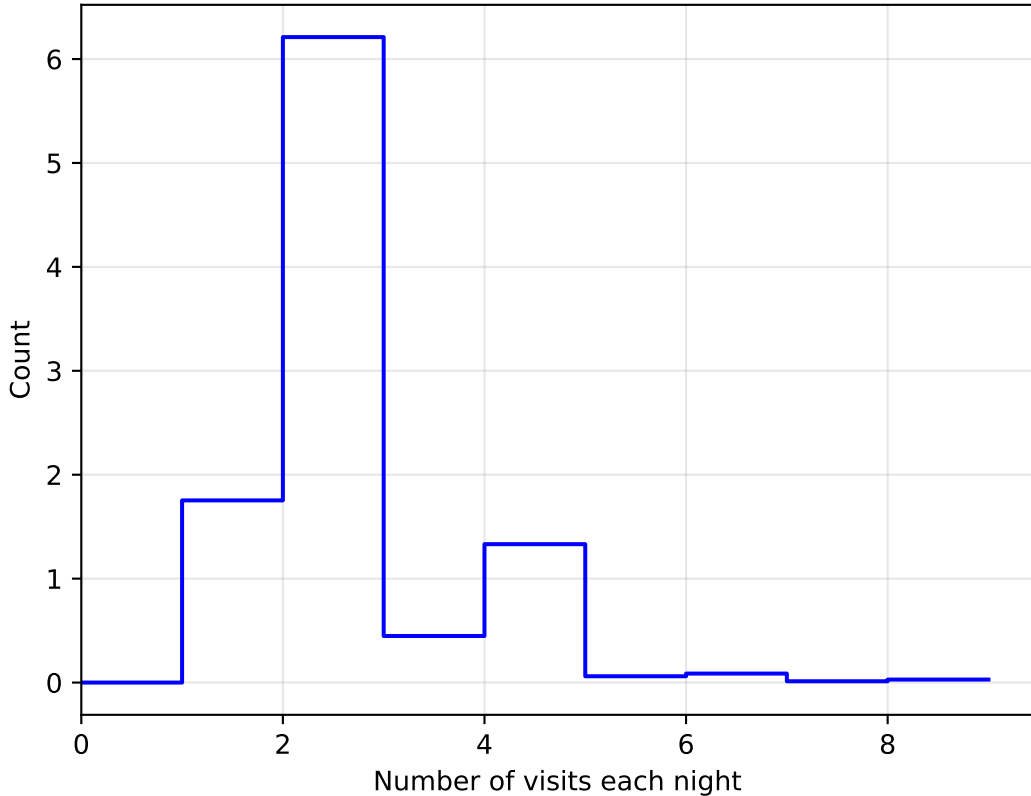
early_u_fpextra3.0_v3.4_10yrs All sky: NVisitsPerNight
