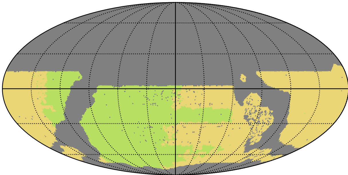
early_u_fpextra3.0_v3.4_10yrs WFD all bands: NSeasons
