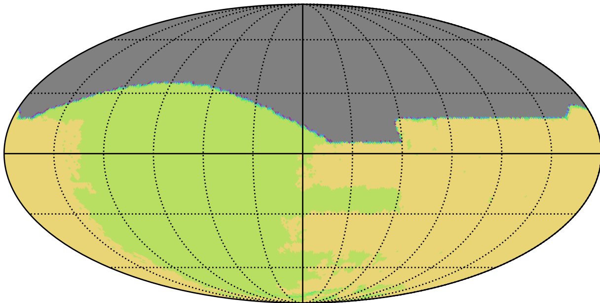
early_u_fpextra3.0_v3.4_10yrs All sky all bands: NSeasons
