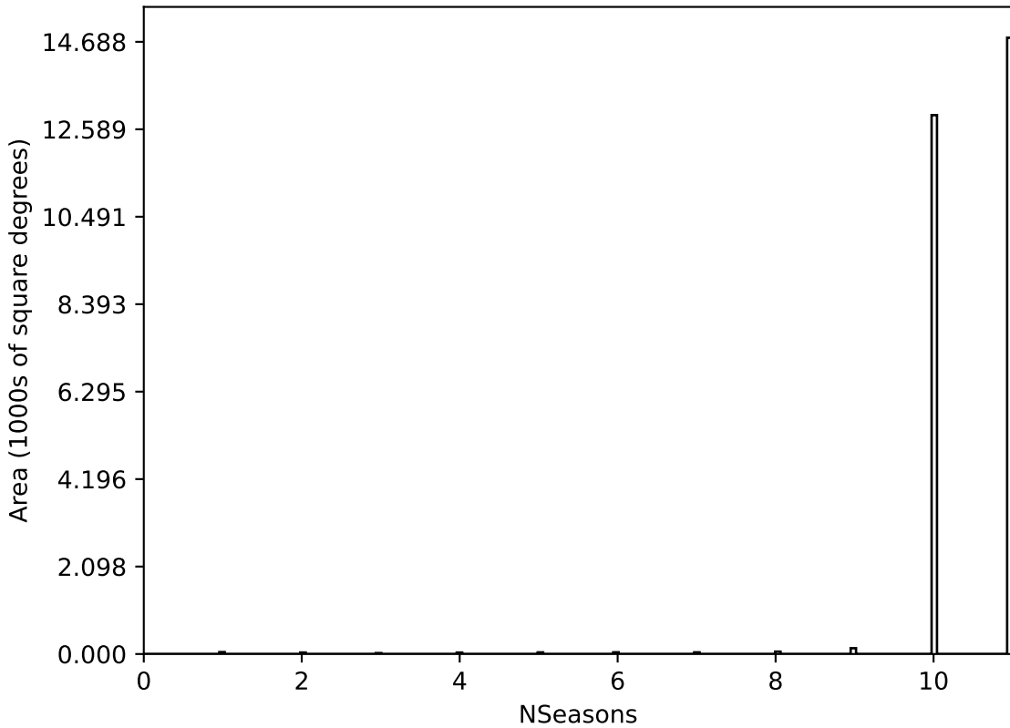
early_u_fpextra3.0_v3.4_10yrs All sky all bands: NSeasons
