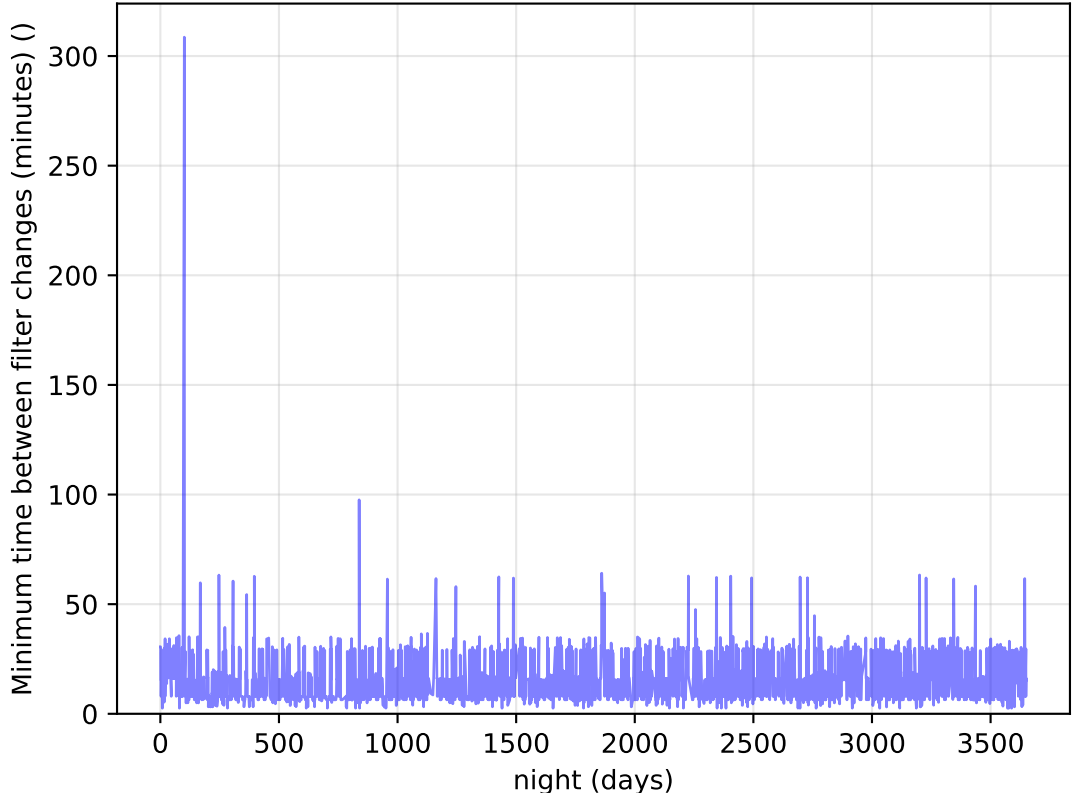
early_u_fpxtra3.0_v3.4_10yrs Per Night: Minimum time between filter changes (minutes)
