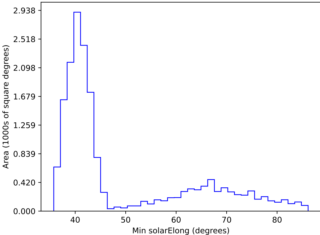
early_u_fpextra3.0_v3.4_10yrs WFD z band: Min solarElong
