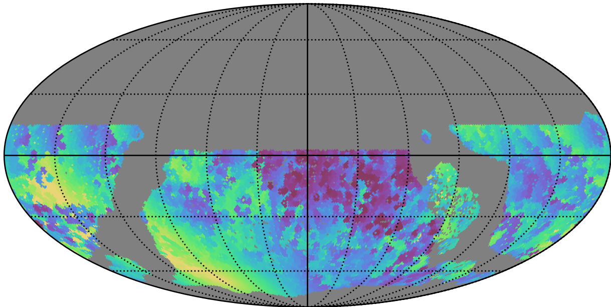
early_u_fpextra3.0_v3.4_10yrs WFD y band: Min solarElong
