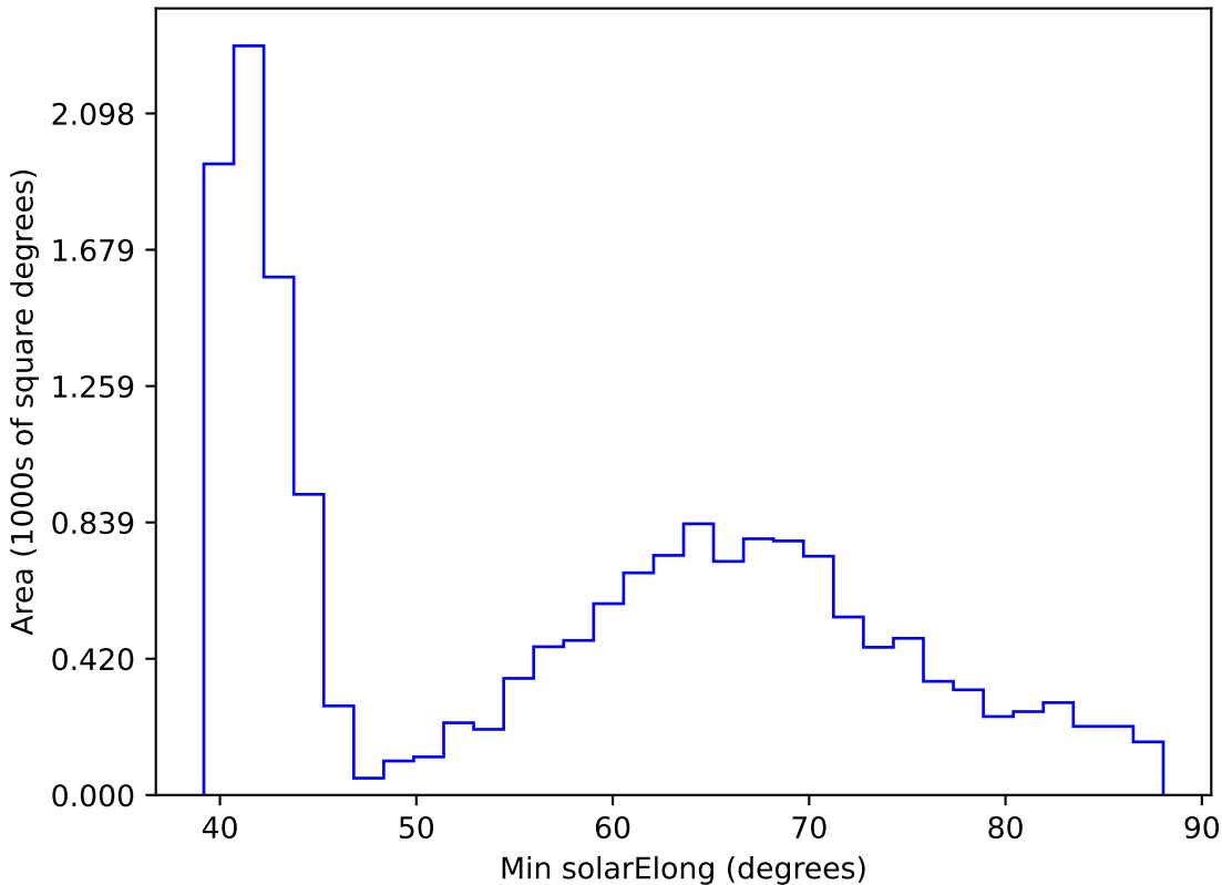
early_u_fpextra3.0_v3.4_10yrs WFD r band: Min solarElong
