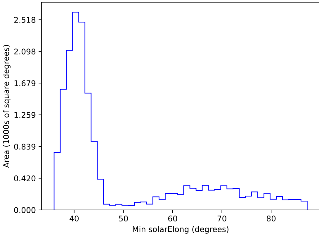
early_u_fpextra3.0_v3.4_10yrs WFD i band: Min solarElong
