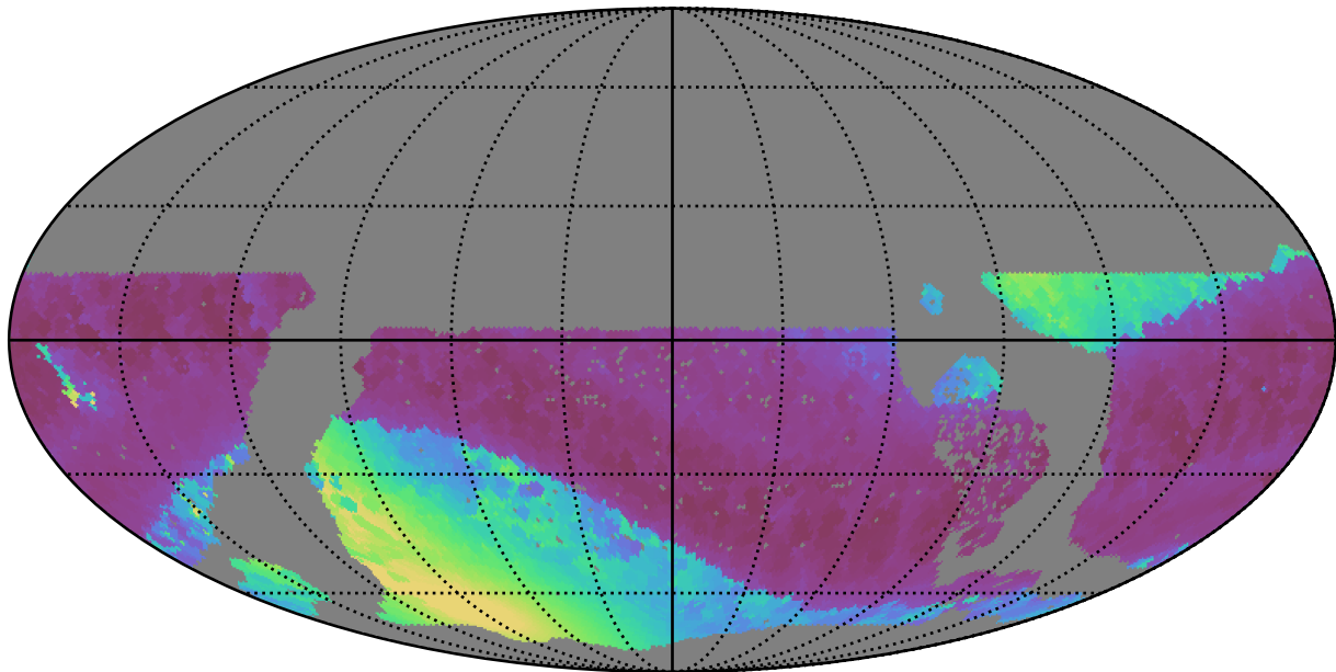
early_u_fpextra3.0_v3.4_10yrs WFD all bands: Min solarElong
