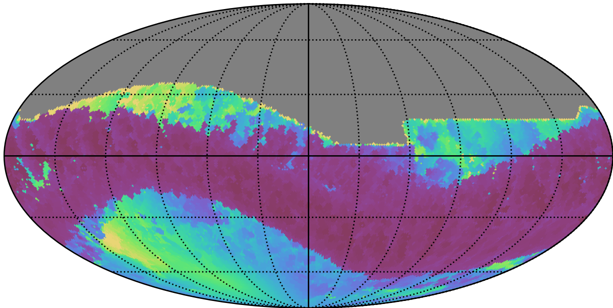
early_u_fpextra3.0_v3.4_10yrs All sky z band: Min solarElong
