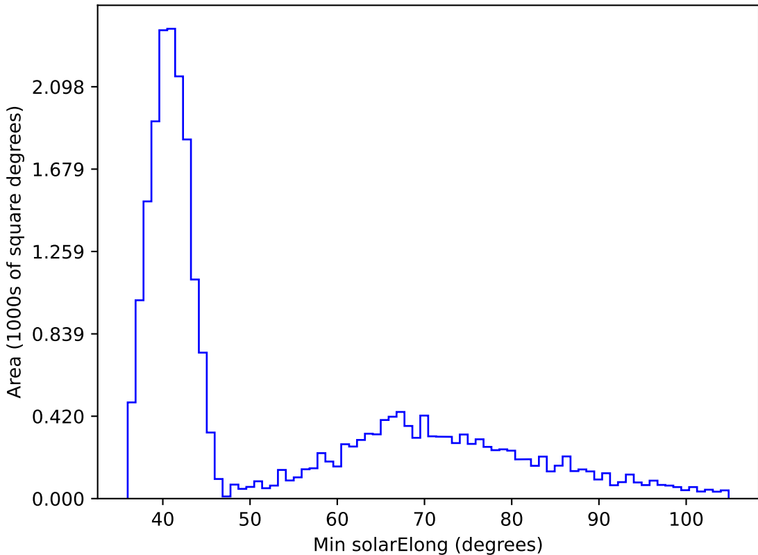
early_u_fpextra3.0_v3.4_10yrs All sky z band: Min solarElong
