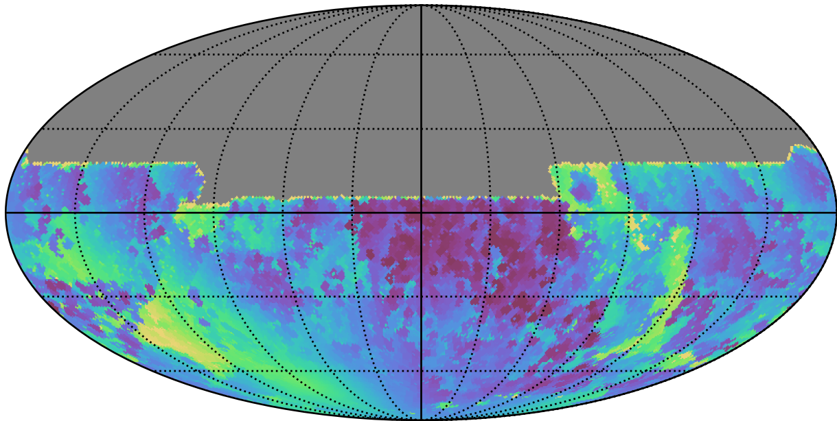
early_u_fpextra3.0_v3.4_10yrs All sky y band: Min solarElong
