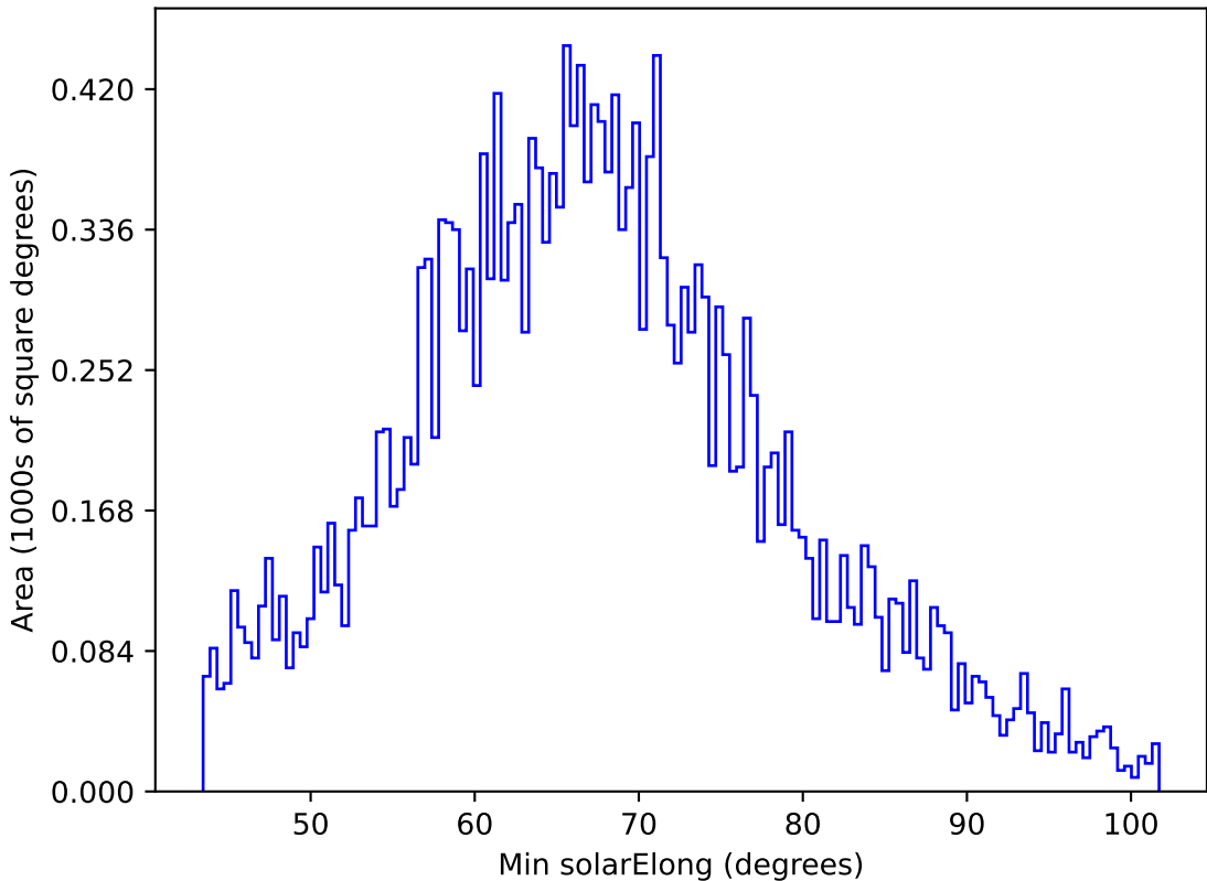
early_u_fpextra3.0_v3.4_10yrs All sky y band: Min solarElong
