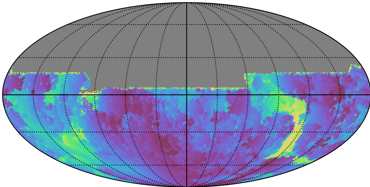
early_u_fpextra3.0_v3.4_10yrs All sky u band: Min solarElong
