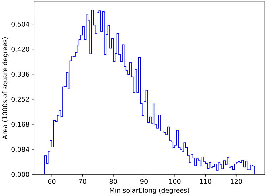
early_u_fpextra3.0_v3.4_10yrs All sky u band: Min solarElong
