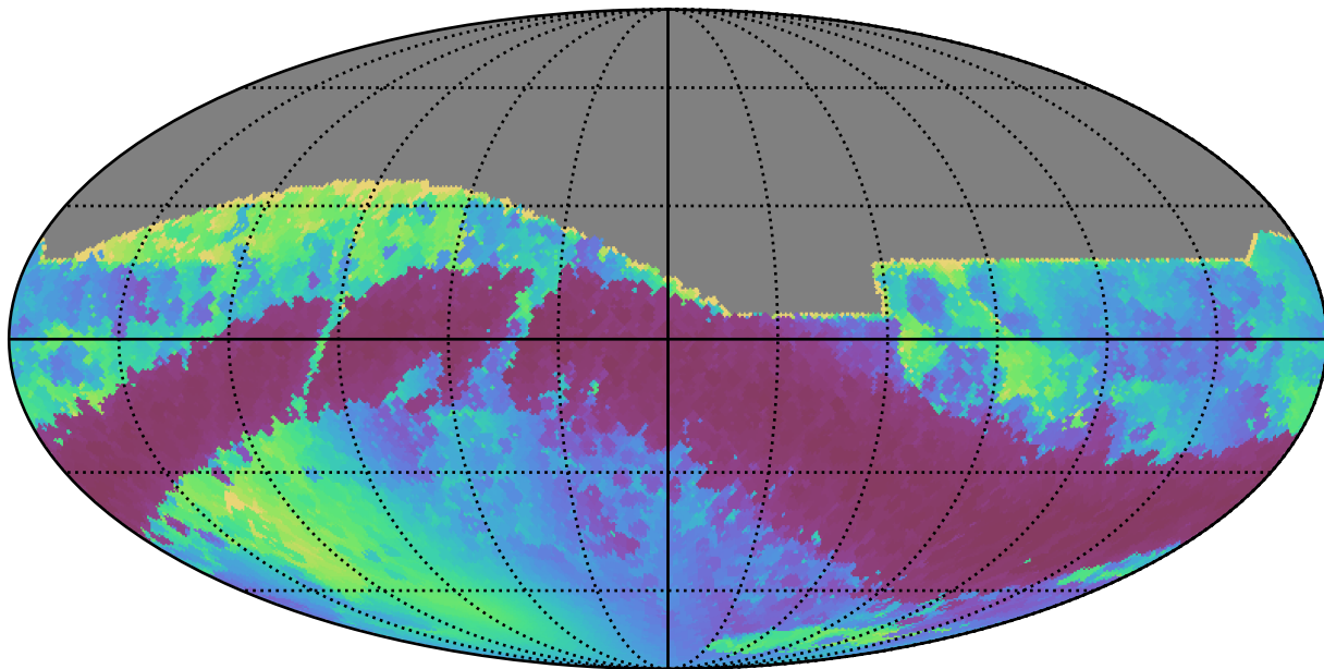
early_u_fpextra3.0_v3.4_10yrs All sky r band: Min solarElong
