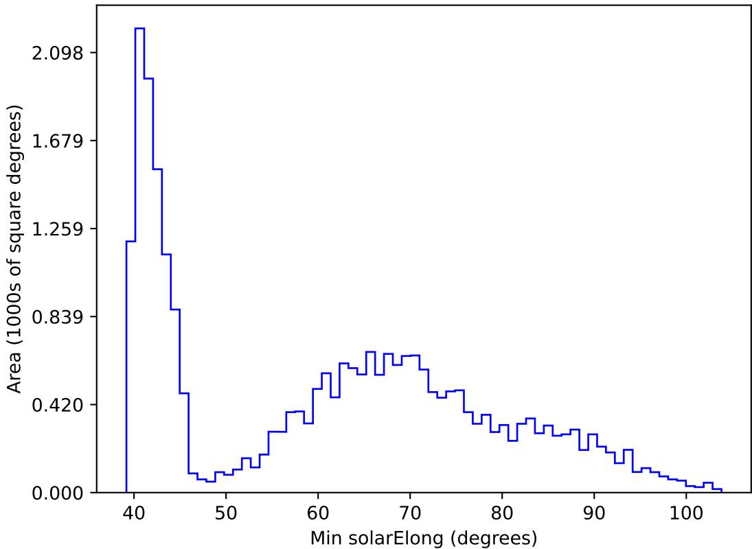
early_u_fpextra3.0_v3.4_10yrs All sky r band: Min solarElong
