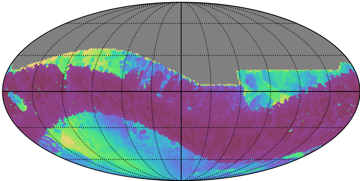
early_u_fpextra3.0_v3.4_10yrs All sky i band: Min solarElong
