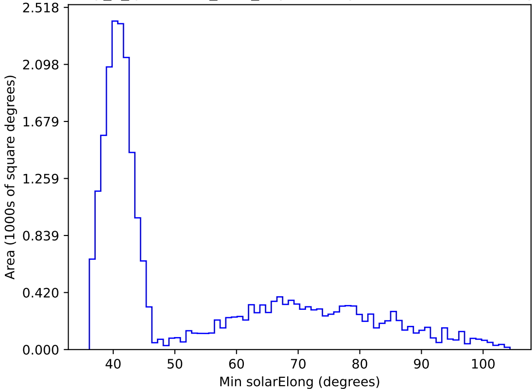
early_u_fpextra3.0_v3.4_10yrs All sky i band: Min solarElong
