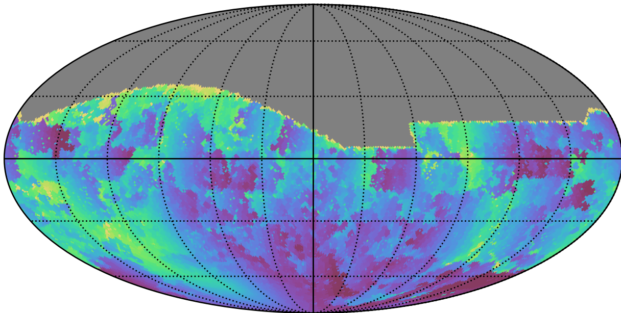
early_u_fpextra3.0_v3.4_10yrs All sky g band: Min solarElong
