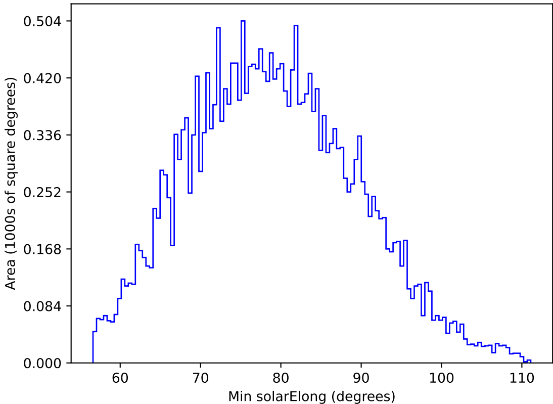
early_u_fpextra3.0_v3.4_10yrs All sky g band: Min solarElong
