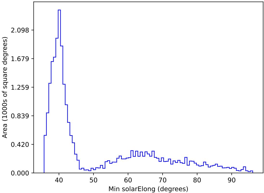
early_u_fpextra3.0_v3.4_10yrs All sky all bands: Min solarElong
