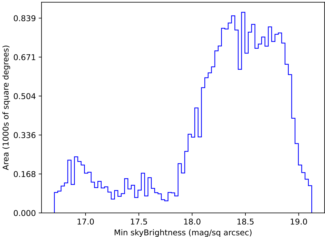
early_u_fpextra3.0_v3.4_10yrs Yr 1 z band: Min skyBrightness
