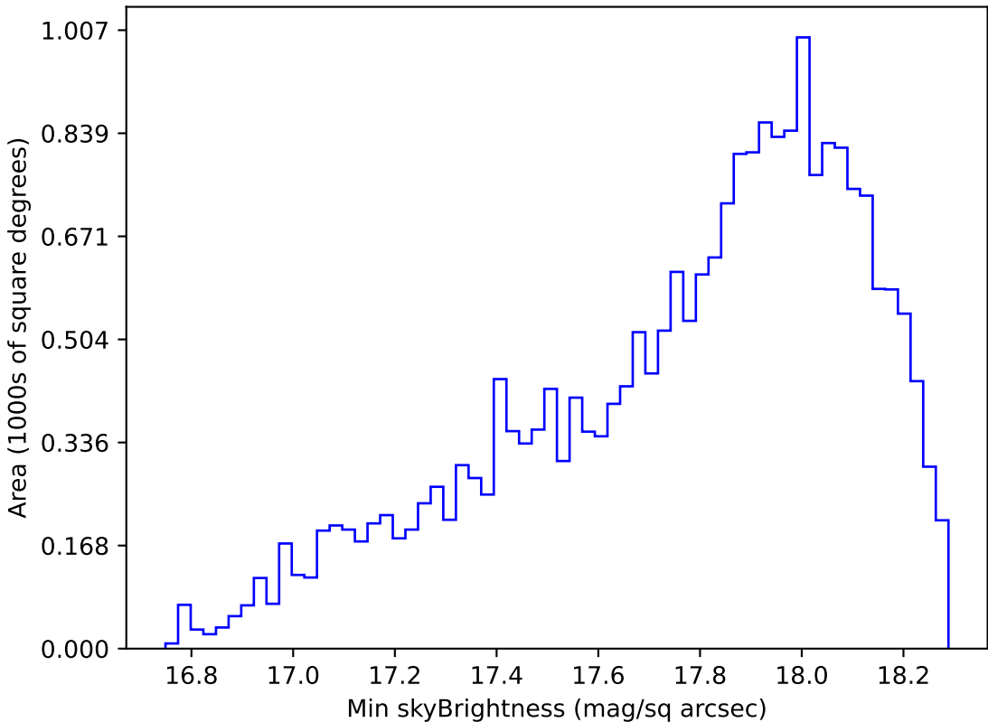
early_u_fpextra3.0_v3.4_10yrs Yr 1 y band: Min skyBrightness
