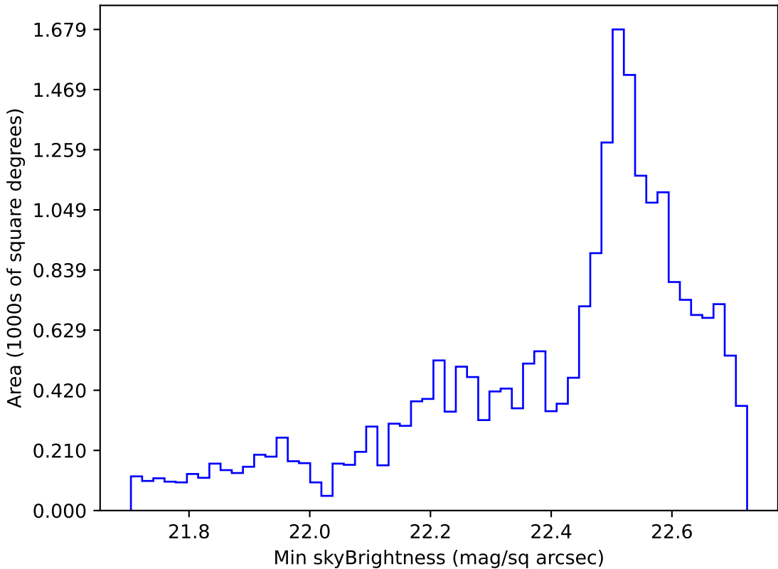
early_u_fpextra3.0_v3.4_10yrs Yr 1 u band: Min skyBrightness
