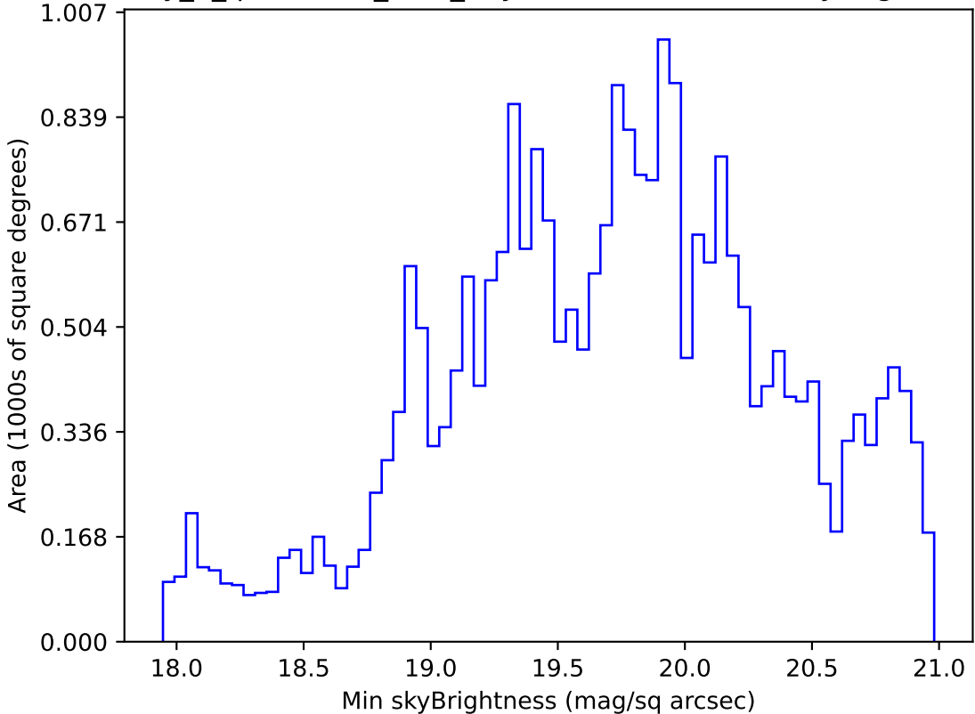
early_u_fpextra3.0_v3.4_10yrs Yr 1 r band: Min skyBrightness
