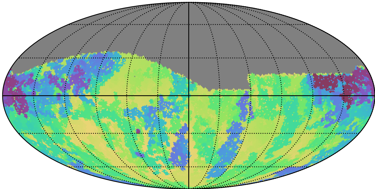
early_u_fpextra3.0_v3.4_10yrs Yr 1 g band: Min skyBrightness
