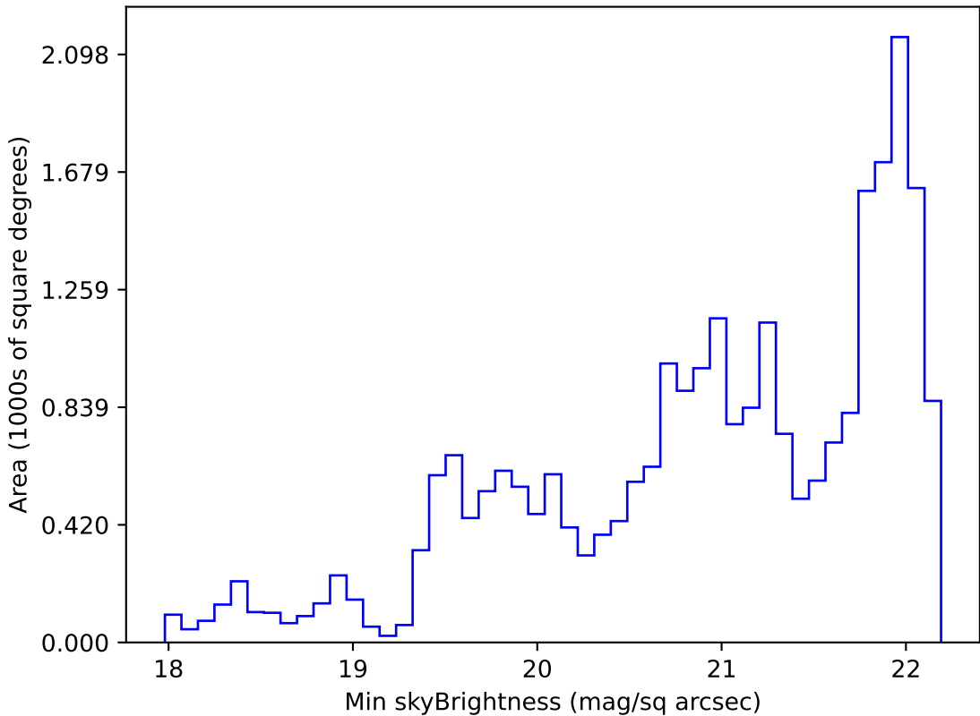
early_u_fpextra3.0_v3.4_10yrs Yr 1 g band: Min skyBrightness
