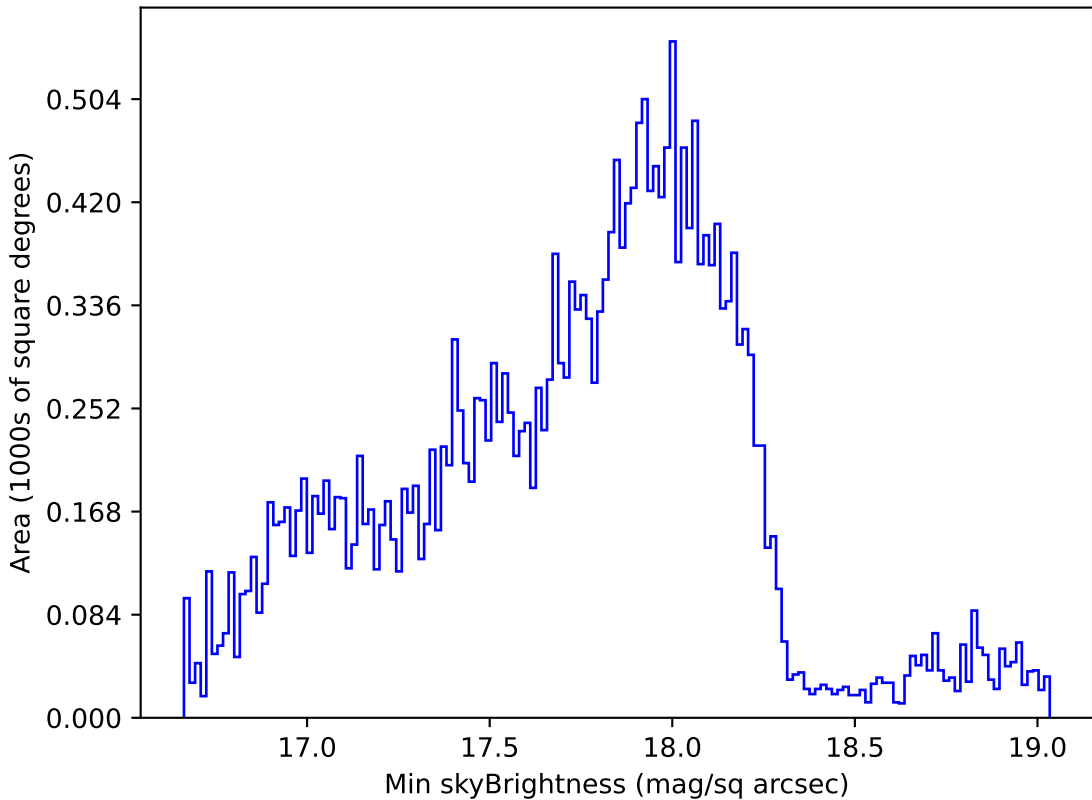
early_u_fpextra3.0_v3.4_10yrs Yr 1 all bands: Min skyBrightness
