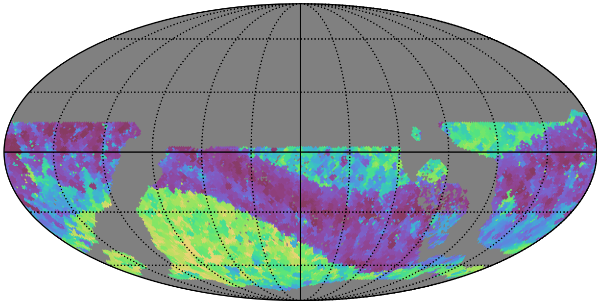
early_u_fpextra3.0_v3.4_10yrs WFD z band: Min skyBrightness
