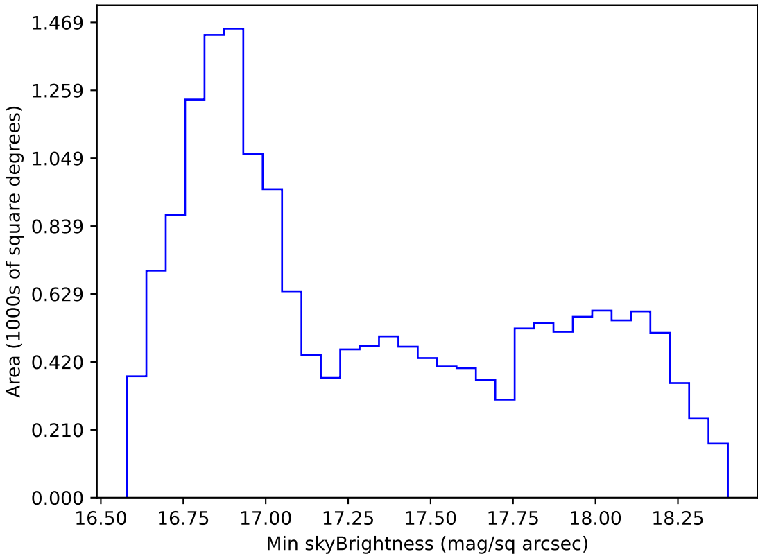
early_u_fpextra3.0_v3.4_10yrs WFD z band: Min skyBrightness
