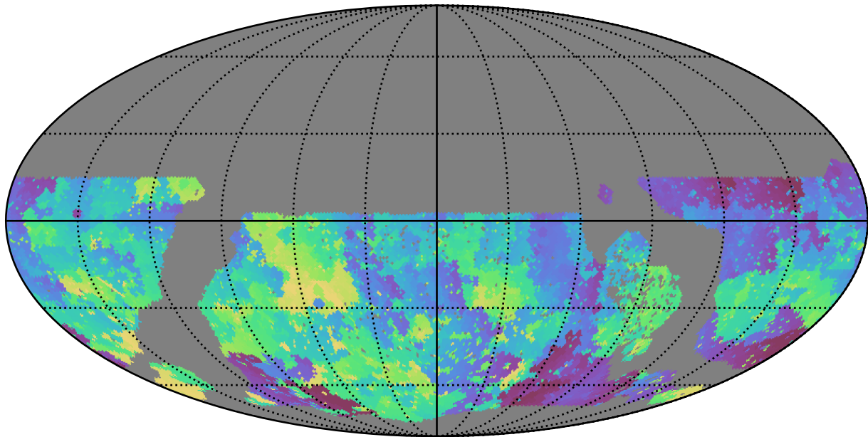
early_u_fpextra3.0_v3.4_10yrs WFD u band: Min skyBrightness
